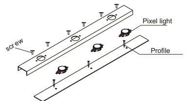
B.Profile installation
