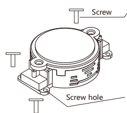
B.Screw installation
