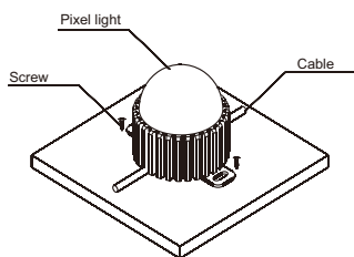
A.Side cable installation
